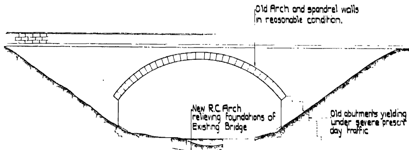
Fig. 210. —Strengthening Foundations of Old Bridge.
